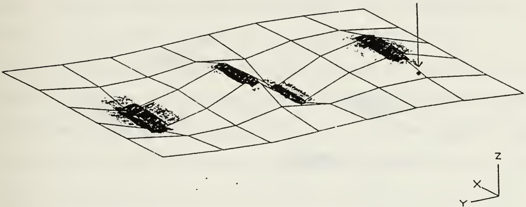
Figure 14. Plate Mode for 1001 Hz (9th Mode). The shaded area represents the highest motion in the plate. The arrow indicates the location of point 6J.
